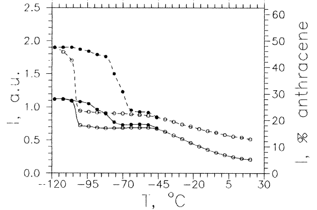
Fig. 8. Light output of pure IPN versus temperature. \circ – for cooling down and \bullet – for heating up; solid lines – in air and dashed lines – in vacuum. Light output of our PS scintillator was taken as 1.
