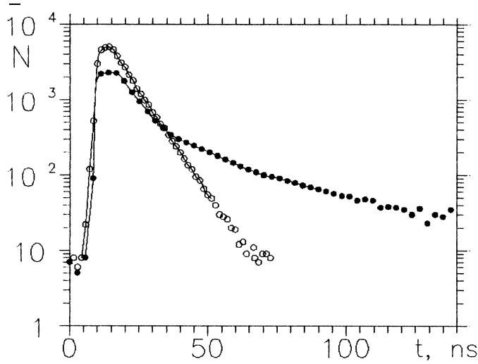
Fig. 11. Decay curves for 1MN + R6. \circ – for T=20^\circ\text{C} in air; \bullet – for T=-120^\circ\text{C} in air.
