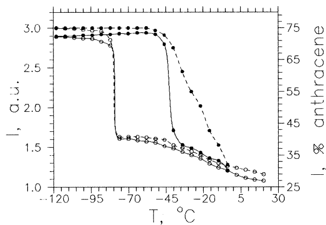
Fig. 6. Light output of 1PN + R6 versus temperature. \circ – for cooling down and \bullet – for heating up; solid lines – in air and dashed lines – in vacuum. Light output of our PS scintillator was taken as 1.
