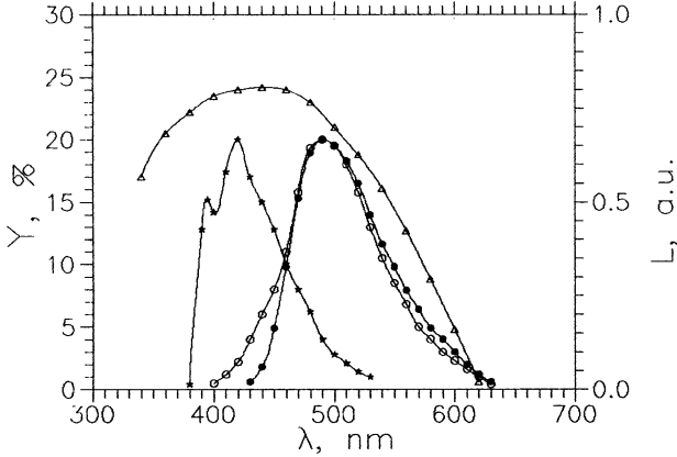
Fig. 1. Quantum efficiency Y of our PM ( \Delta ) and luminescent spectra L of our PS scintillator ( \star ), 1MN + R6 in air at T=20^\circ\text{C} ( \bullet ) and 1MN + R6 in air at T=-120^\circ\text{C} ( \circ ) for the excitation at 365 nm.
