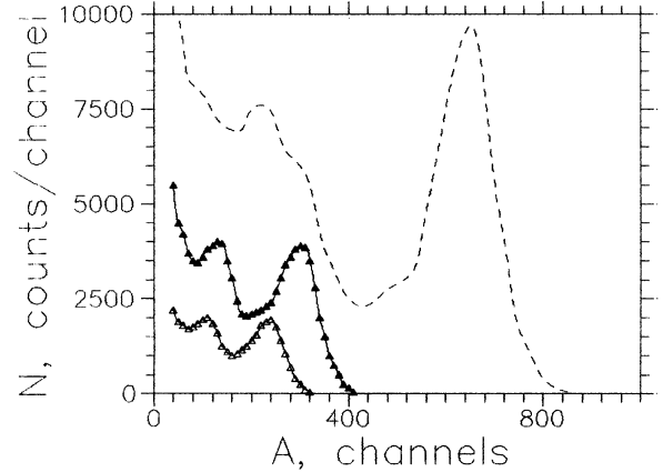
Fig. 2. Pulse height spectra of scintillation signals from ^{207}\text{Bi} in IPN + R6 (solid lines) and anthracene (dashed line). \Delta – at 20^\circ\text{C} in air; \blacktriangle – at 20^\circ\text{C} in vacuum.
