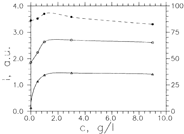
Fig. 9. Light output of 1MN + R6 versus the dopant concentration. \Delta – for T=20^{\circ}\text{C} in air; \circ – for T=-120^{\circ} in air; \bullet – for T=-120^{\circ}\text{C} in vacuum.
