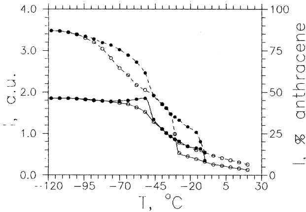
Fig. 7. Light output of pure 1MN versus temperature. \circ – for cooling down and \bullet – for heating up; solid lines – in air and dashed lines – in vacuum. Light output of our PS scintillator was taken as 1.
