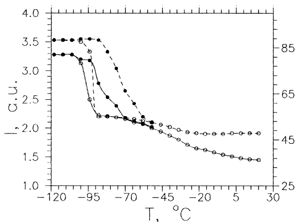
Fig. 5. Light output of IPN + R6 versus temperature. \circ – for cooling down and \bullet – for heating up; solid lines – in air and dashed lines – in vacuum. Light output of our PS scintillator was taken as 1.
