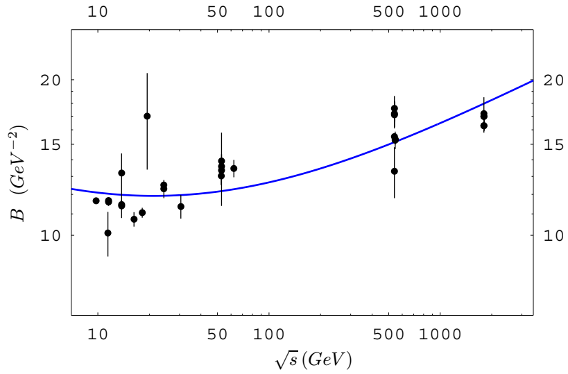
Figure 3: Slope B of diffraction cone in p\bar{p} elastic scattering. Solid line represents our fit to the data.
