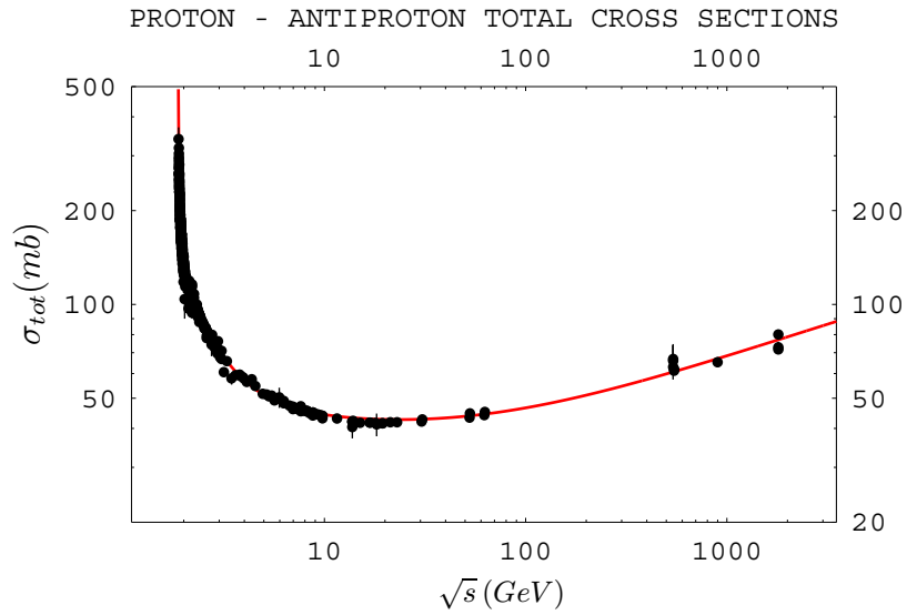
Figure 4: The total proton-antiproton cross-section versus \sqrt{s} compared with formula (49). Solid line represents our fit to the data.
