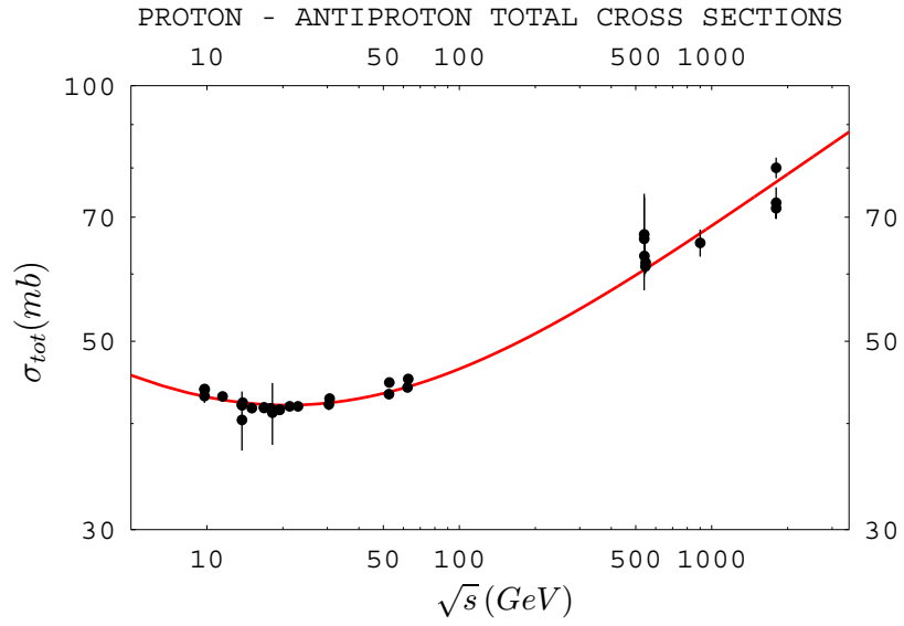
Figure 2: The total proton-antiproton cross-section versus \sqrt{s} compared with formula (44). Solid line represents our fit to the data. Statistical and systematic errors added in quadrature.
