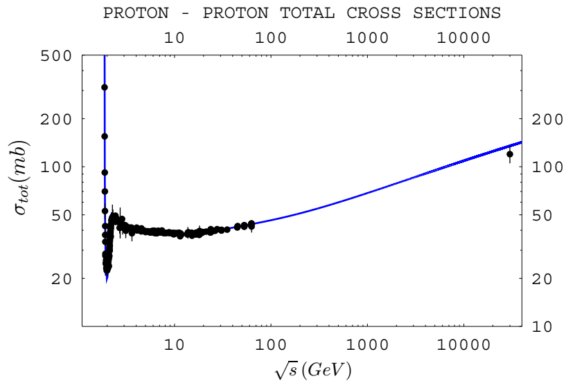
Figure 7: The total proton-proton cross-section (vs \sqrt{s} ) including point from cosmic rays experiment [33] compared with formula (56). Solid line represents our fit to the data.
