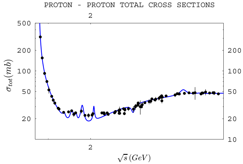
Figure 9: The total proton-proton cross-section at low energies compared with formula (56). Solid line represents our fit to the data.
