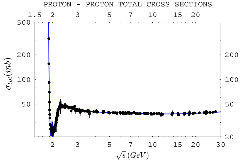
Figure 8: The total proton-proton cross-section in the range \sqrt{s} < 30 GeV compared with formula (56). Solid line represents our fit to the data.
