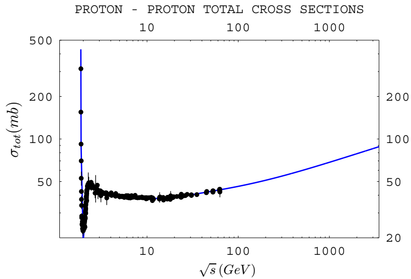
Figure 6: The total proton-proton cross-section versus \sqrt{s} compared with formula (56). Solid line represents our fit to the data. Statistical and systematic errors added in quadrature.
