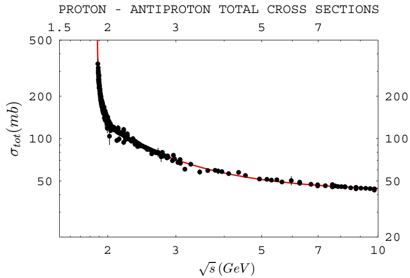
Figure 5: The total proton-antiproton cross-section versus \sqrt{s} compared with formula (49) in the range \sqrt{s} < 10 GeV (fragment of Fig. 4). Solid line represents our fit to the data.
