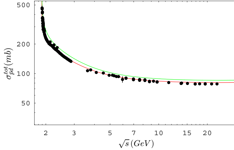
Figure 8: The total antiproton-deuteron cross-section versus \sqrt{s} compared with the theory with and without shadow corrections.
