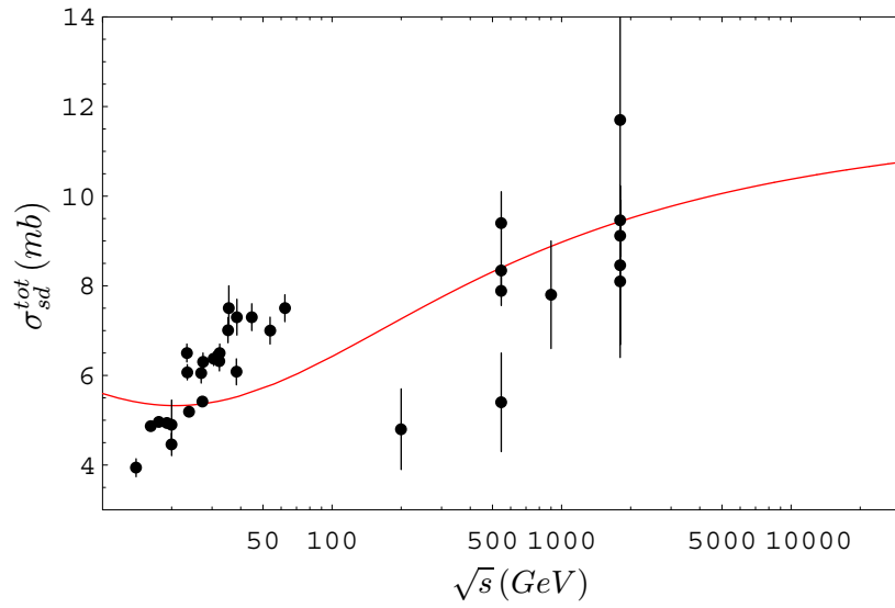
Figure 3: Total single diffraction dissociation cross-section compared with formula (37). Solid line represents our fit to the data.
