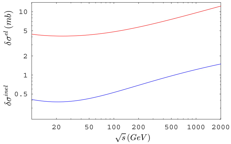
Figure 9: Elastic and inelastic shadow corrections (vs \sqrt{s} ) represented by the theory.
