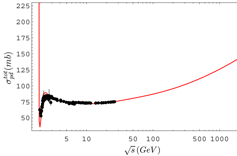
Figure 5: The total proton-deuteron cross-section versus \sqrt{s} compared with the theory without any free parameters. Statistical and systematic errors added in quadrature.
