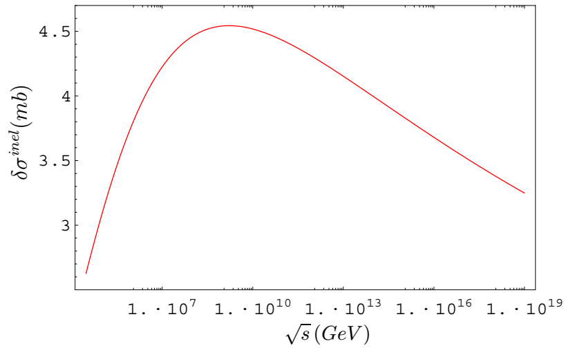
Figure 7: The three-body forces contribution (inelastic screening) to the total antiproton-deuteron cross-section calculated with the theory in the range 30000 GeV < \sqrt{s} < 10^{19} GeV .
