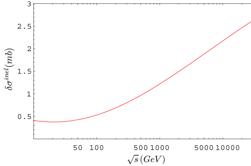
Figure 6: The three-body forces contribution (inelastic screening) to the total antiproton-deuteron cross-section versus \sqrt{s} calculated with the theory.
