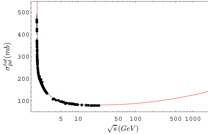
Figure 4: The total antiproton-deuteron cross-section versus \sqrt{s} compared with the theory. Statistical and systematic errors added in quadrature.
