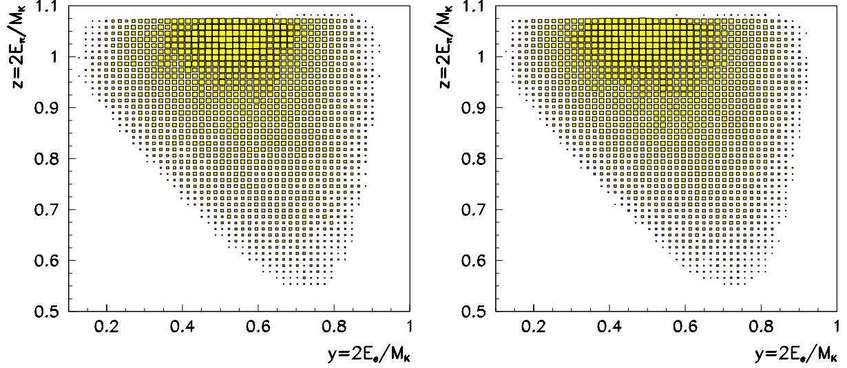
Fig. 6. Dalitz plots ( y = 2E_e/M_K ; z = 2E_{\pi^0}/M_K ) for the selected K^- \rightarrow e^- \nu \pi^0 events after the 2-C fit. Left — 1999 statistics, right — 2001 statistics.
