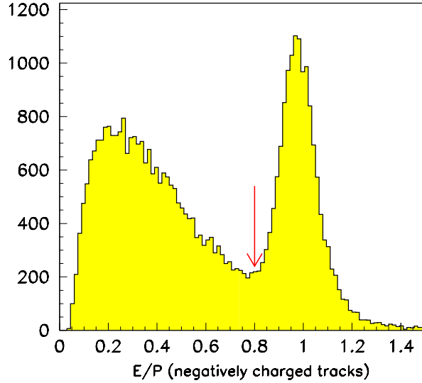
Fig. 2. The E/p plot — the ratio of the energy of the associated cluster in ECAL to the momentum of the charged track. The arrow shows the cut used for the electron separation.
