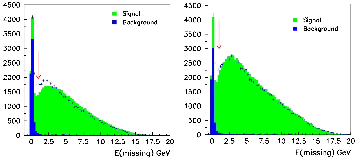
Fig. 5. The missing energy for the e\pi^0 events, for 1999 run (left) and 2001 run (right). The points with errors are the data, the histograms — MC. The dark(blue) peak at zero value corresponds to the MC-predicted K^- \rightarrow \pi^- \pi^0 background. The arrow indicates the cut value.
