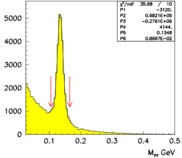
Fig. 3. The \gamma\gamma mass spectrum for the events with the identified electron and two extra showers.
