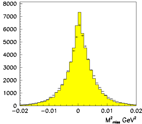
Fig. 4. The missing four-momentum squared (P_K - P_e - P_{\pi^0})^2 for the selected events for 1999 run (left) and 2001 run (right). The points with errors are the data, the histogram — MC.
