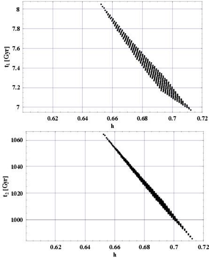
Figure 2. The dependences of the time of the beginning of the Universe accelerated expansion (a) and its cessation (b) on the h value for \nu = 0.05 at \Omega_{\text{tot}} = 1.04 ; 13.5 < t_0 < 13.9 GY; \nu = 0.05 ; 0.126 < \omega_m < 0.143 .
