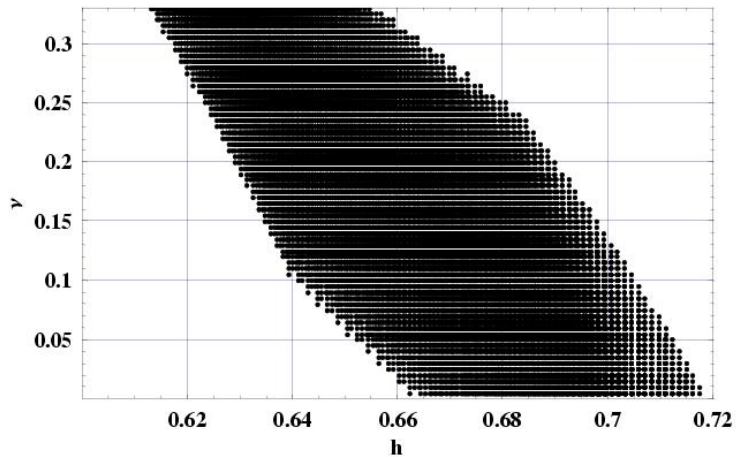
Figure 1. The range of the \nu parameter variation for \Omega_{\text{tot}} = 1.04 ; 0.126 \leq \omega_m \leq 0.143 , 13.5 < t_0 < 13.9 GY.
