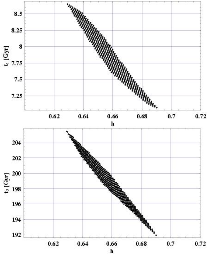
Figure 3. The same as in Fig. 2, but for \nu = 0.20 .
