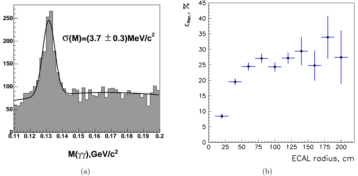
Figure 4. The \pi^0 signal in the \gamma\gamma spectrum from B^0 \rightarrow \rho^+\pi^- simulated events (a) and the efficiency of reconstructing the \pi^0 as a function of distance from the beam line (b). All events considered have at least one signal B decay. The sample includes a mean of two Poisson distributed non-beauty interactions per beam crossing.
