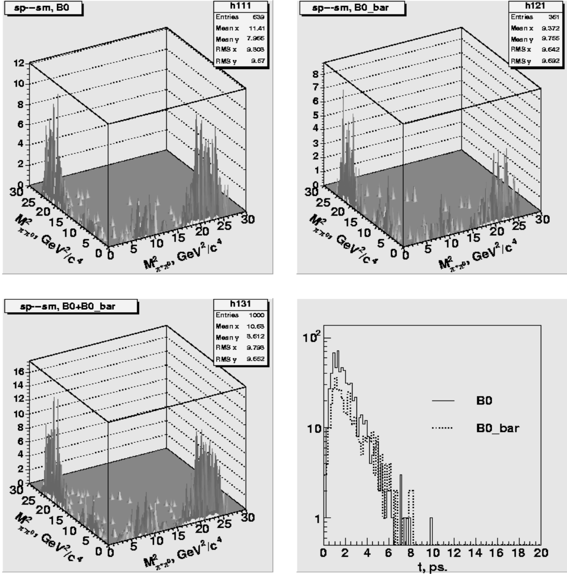
Figure 9. Dalitz-plot and proper time distribution for one trial of 1000 events for \alpha = 88^\circ (detector efficiency included).
