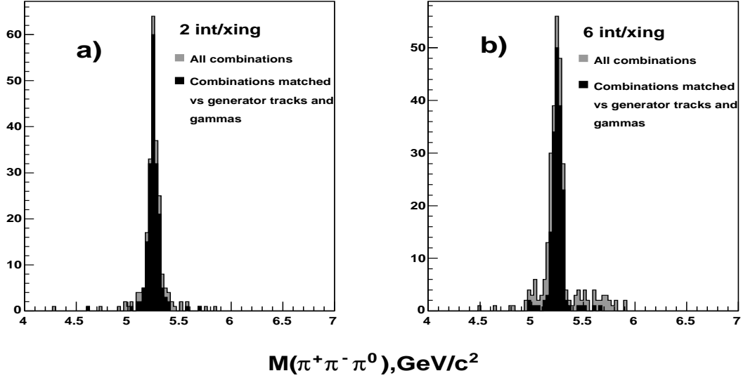
Figure 6. Invariant mass \pi^+\pi^-\pi^0 (after cuts) matched vs generator tracks and photons, for the simulated B^0 \rightarrow \rho^+\pi^- at 2 and 6 interactions per crossing.
