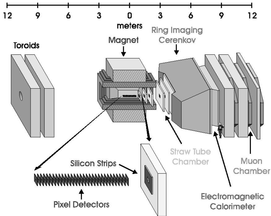
Figure 3. Layout of the BTeV Detector.
