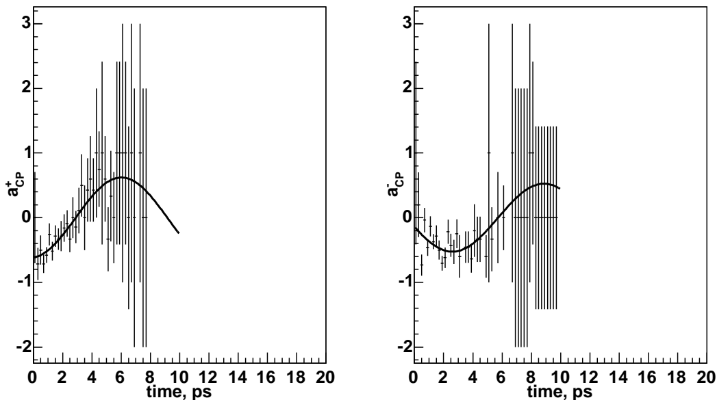
Figure 11. CP-asymmetries a_{cp}^+ for \rho^+\pi^- and a_{cp}^- for \rho^-\pi^+ . The solid curves represent the fit.
