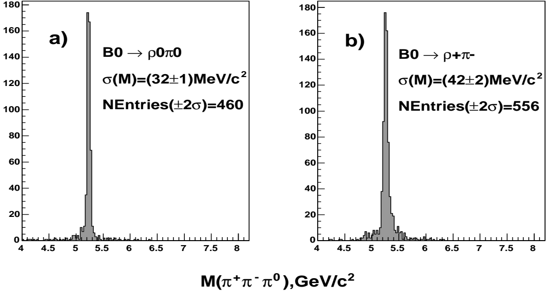
Figure 5. Invariant mass \pi^+\pi^-\pi^0 (after cuts) for the simulated (a) B^0 \rightarrow \rho^0\pi^0 and (b) B^0 \rightarrow \rho^+\pi^- decays. Each event includes on the average two Poisson distributed non-beauty interactions per beam crossing, mixed to the beauty production interaction. The number of signal event were counted as the number of entries in the \pm 2\sigma interval around the B mass, minus estimated number of background entries.
