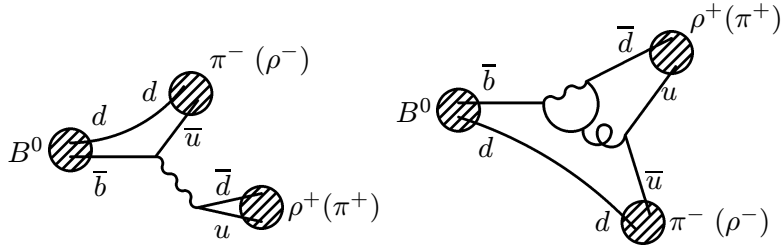
Figure 8. The tree (left) and penguin (right) diagrams for the B^0 \rightarrow \rho^+ \pi^- ( B^0 \rightarrow \rho^- \pi^+ ) decays.
