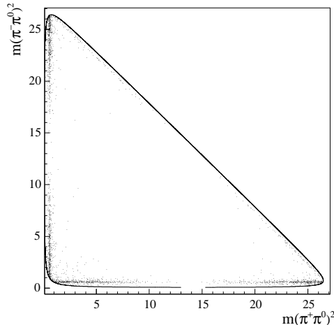
Figure 2. The Dalitz plot for B^0 \rightarrow \rho\pi \rightarrow \pi^+\pi^-\pi^0 .
