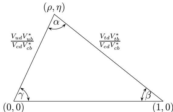
Figure 1. Unitary Triangle.
