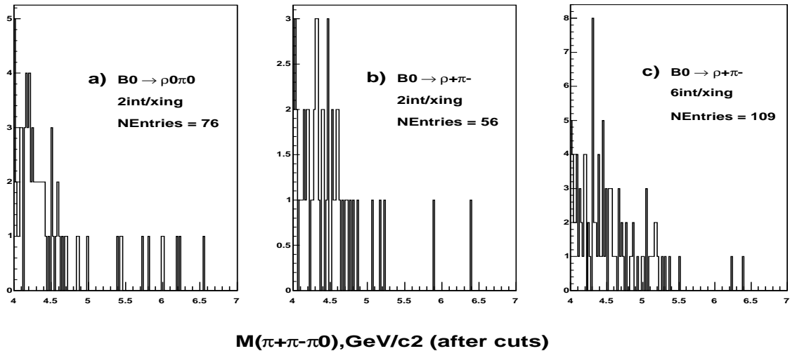
Figure 7. Background \pi^+\pi^-\pi^0 invariant mass for B^0 \rightarrow \rho^0\pi^0 and B^0 \rightarrow \rho^+\pi^- at 2 interactions per crossing (a,b), and B^0 \rightarrow \rho^+\pi^- at 6 interactions per crossing (c).
