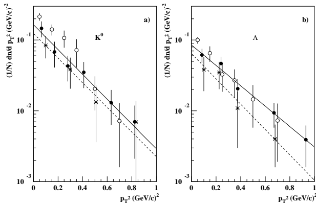
Figure 7. The p_T^2 -distributions of K^0 (a) and \Lambda (b) in the 'quasinucleon' subsample (asterisks), at A_{eff} \approx 21 (black circles) and A_{eff} \approx 45 (open circles). The curves are the result of the exponential fit for the 'quasinucleon' subsample (dashed) and for A_{eff} \approx 21 (solid).
