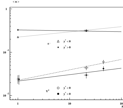
Figure 2. The A-dependence of the yields of V^0 , and \pi^- in the forward ( y^* > 0 ) and backward ( y^* < 0 ) hemispheres and of the total yield of V^0 . The curves are the result of the exponential fit.
