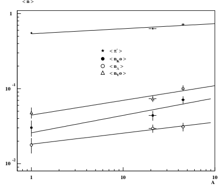
Figure 1. The A-dependence of the total yields of K^0 , \Lambda and \pi^- . The curves are the result of the exponential fit.
