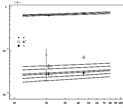
Figure 8. The A-dependence of the total yields of K^0 (open circles), \Lambda (black circles) and \pi^- (asterisks). The solid and dashed curves are the model predictions and the uncertainty in the latter (see text)
