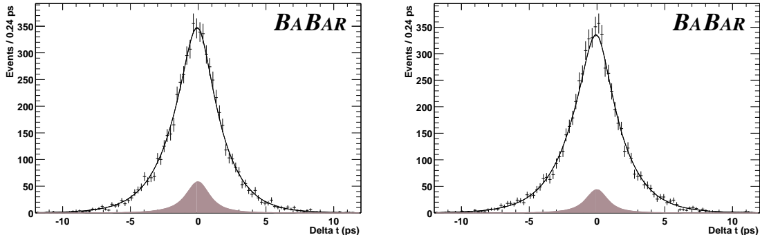
Fig. 2. \Delta t distributions for B^0/\bar{B}^0 (left) and B^+/B^- (right) candidates in the signal region ( m_{ES} > 5.27 \text{ GeV}/c^2 ). The result of the lifetime fit is superimposed. The background is shown by the hatched area.
