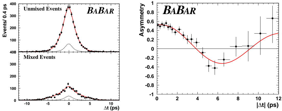
Fig. 4. \Delta t distribution for mixed and unmixed events (left) and the time-dependent asymmetry a(\Delta t) between unmixed and mixed events (right).
