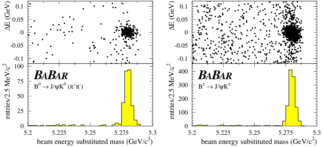
Fig. 1. Example distribution of the candidates in the \Delta E – m_{ES} plane for B^0 \rightarrow J/\psi K_s^0 and B^\pm \rightarrow J/\psi K^\pm .
