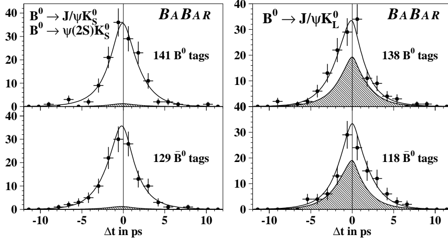
Fig. 3. Distribution of \Delta t for the B^0 and \bar{B}^0 tags. Shown on the left for B^0 \rightarrow J/\psi K_S^0 and B^0 \rightarrow \psi(2S)K_S^0 , and on the right for B^0 \rightarrow J/\psi K_L^0 . The background which is significantly larger for the K_L^0 mode is shown by the hatched area.
